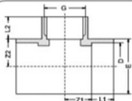
TEE 90° FEMALE THREADED SOLVENT GLUING
